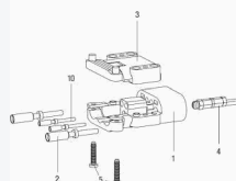
PLUG (MALE) · NUMBERS = POS. IN THE TABLES
