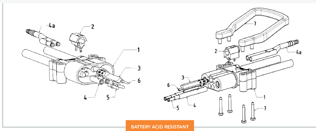
MRC 320/400 PLUG AND SOCKET – DRAWING © REMA · NUMBERS = POS. IN THE TABLES
